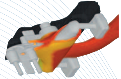
Metal front progression around a core
