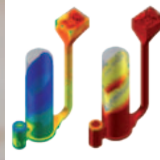
Trial run of partially filled prototype casting vs. Simulation results showing favorable correlation.
